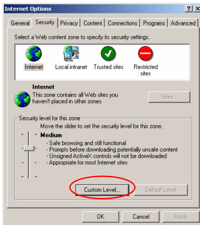
Figure 119 Internet Options
