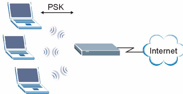
Figure 154 WPA(2)-PSK Authentication
