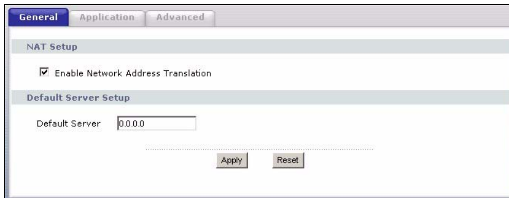
Figure 75 NAT General
