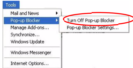
Figure 115 Pop-up Blocker
