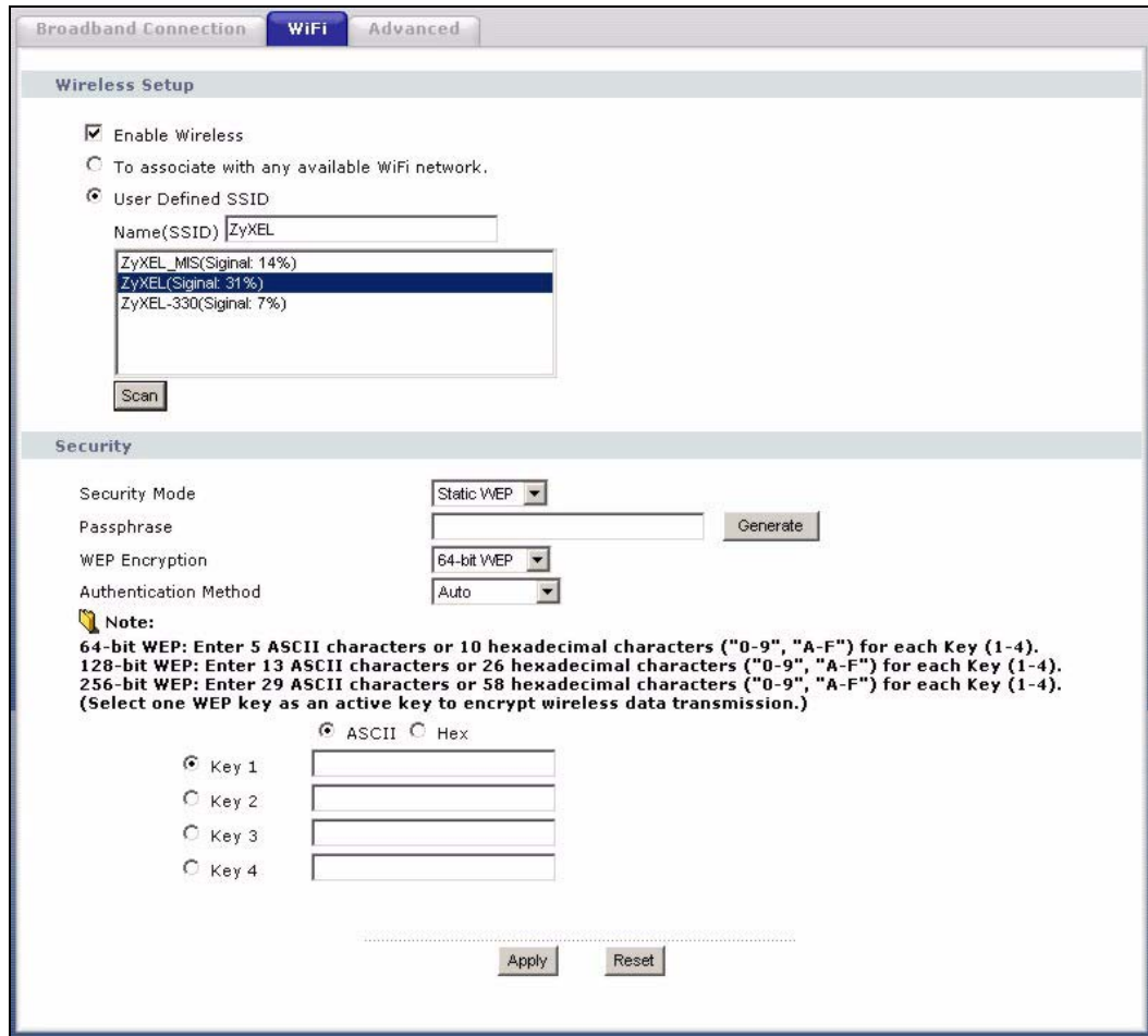
Figure 65 WiFi: Static WEP Encryption
