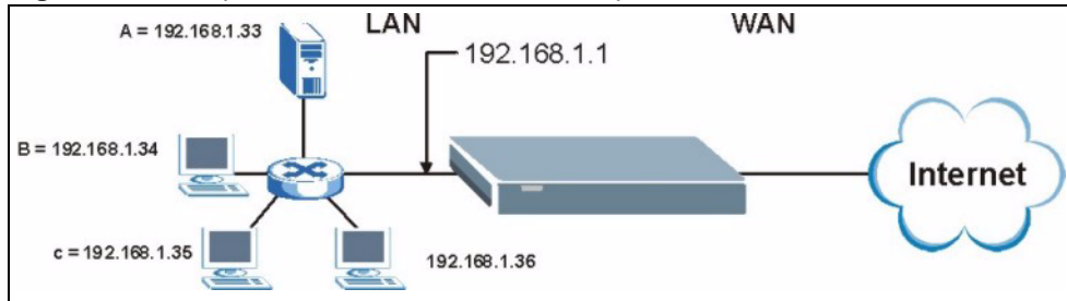
Figure 74 Multiple Servers Behind NAT Example
