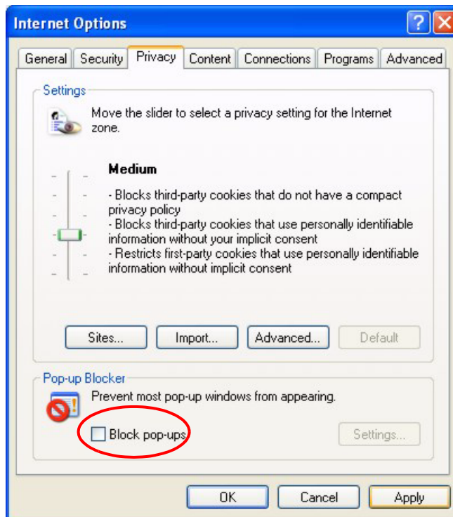
Figure 116 Internet Options
