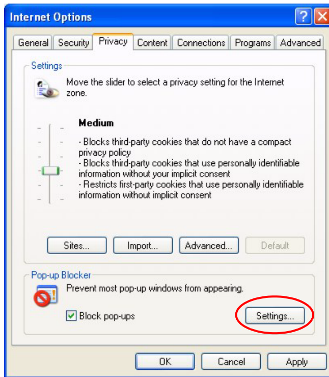
Figure 117 Internet Options
