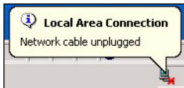
Figure 111 Temporarily Disconnected
